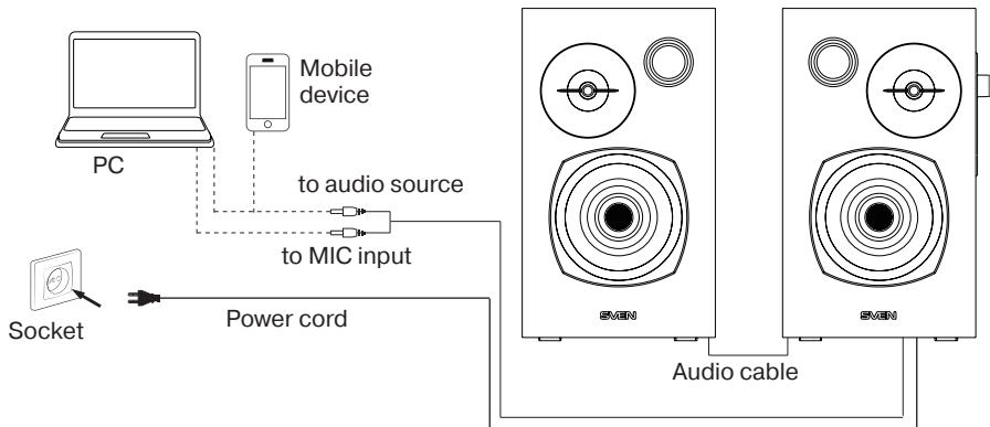
Fig. 2. Connection diagram
